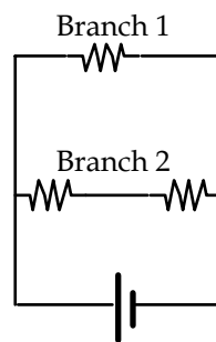
Figure 2.7: This circuit represents a parallel-series combination
