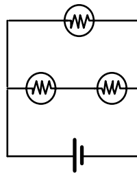
Circuit 3
