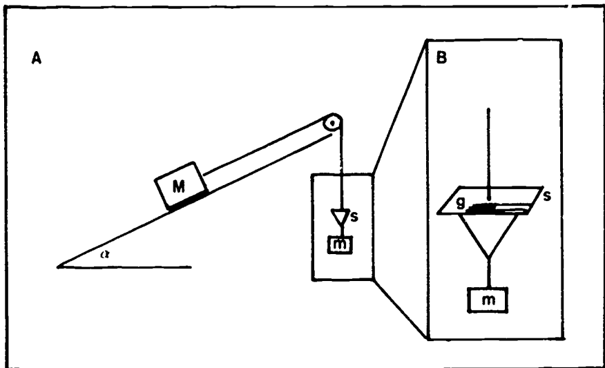
Figure 1. (A) The experiment set-up. (B) Detail of the leaf spring s with strain gauge g glued on top.
