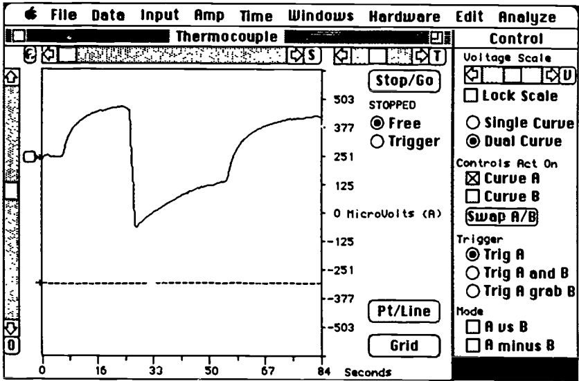
Figure 3. With amplification up to a factor of 64,000 times, we do not need an external amplifier to make direct readings of a thermocouple, seen here as curve A. We have displayed the dual beam controls, but here there is no input for curve B (dotted line).
