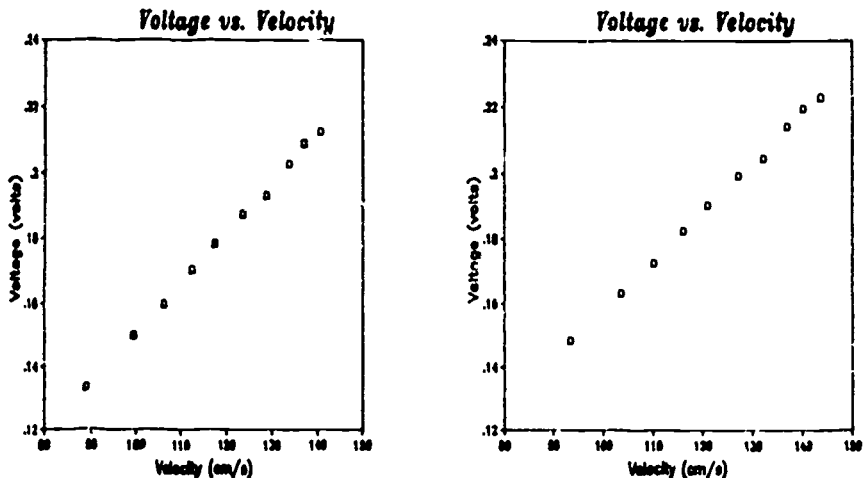
Figure 13. Voltage versus velocity using Faraday's law apparatus.
