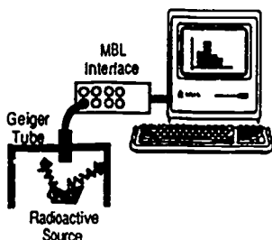
(a) MBL based nuclear radiation counting system for the Mac Computer.
