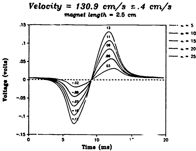
Figure 12. Voltage versus time using Faraday's law apparatus.
