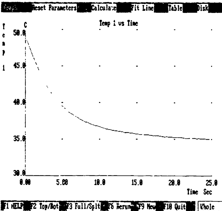
Figure 5. A cooling curve taken with the PSL Toolkit .
