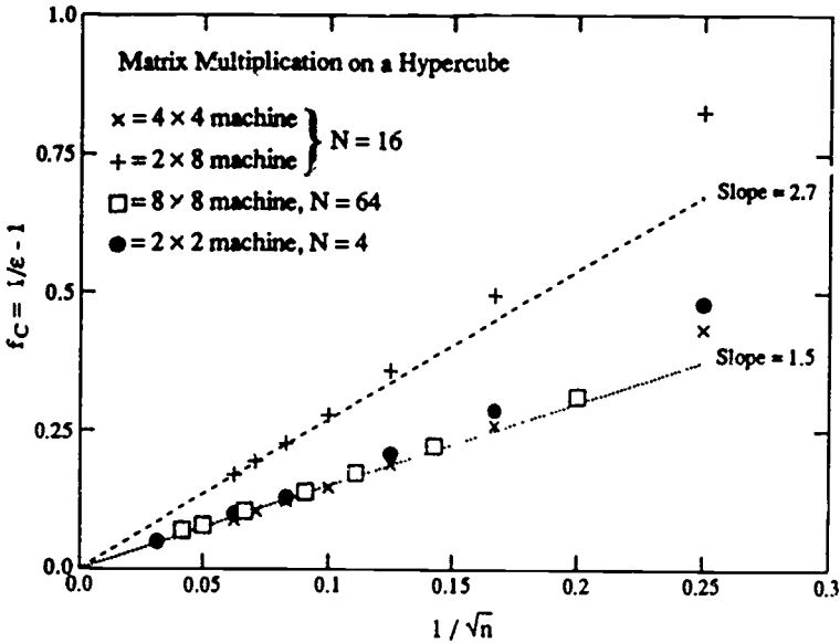
Figure 6. Experimentally measured overhead f_C for the multiplication of two M \times M matrices on a hypercube. The number of matrix elements per node n is given by n = (M^2)/N . For this problem the system dimension d is 2. The dashed lines show the asymptotic behavior for large n . Note that f_C is independent of N for a square decomposition.
