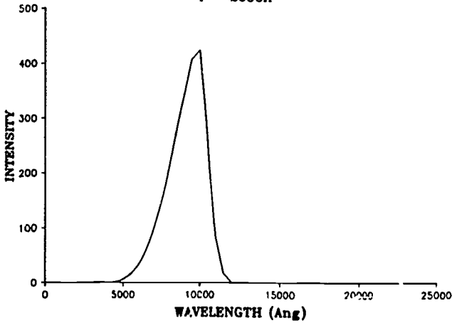
Figure 4. Response function of a photodiode to an incandescent source.
