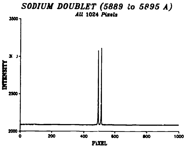
Figure 9. Visible spectrum for Na showing the doublet lines.
