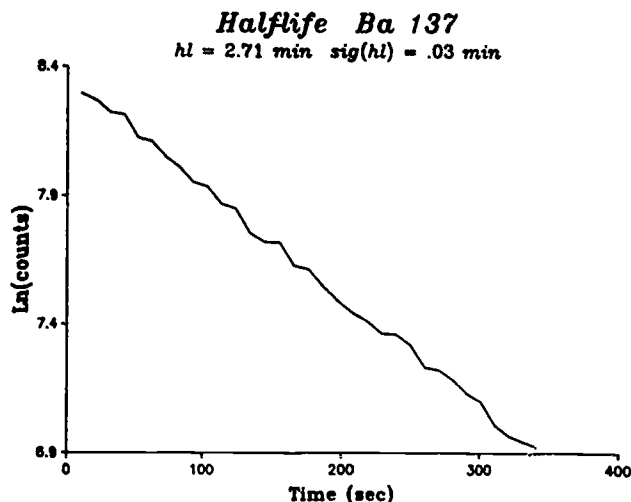
Figure 6. Decay curve for Ba^{137} .
