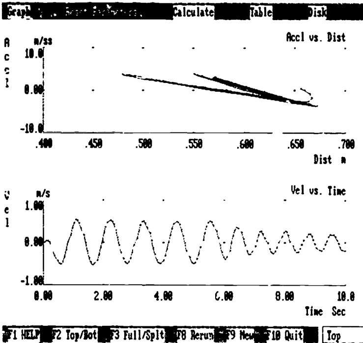
Figure 3. PSL Toolkit , showing two graphs of the same event, one displaying acceleration against position and the other velocity against time.
