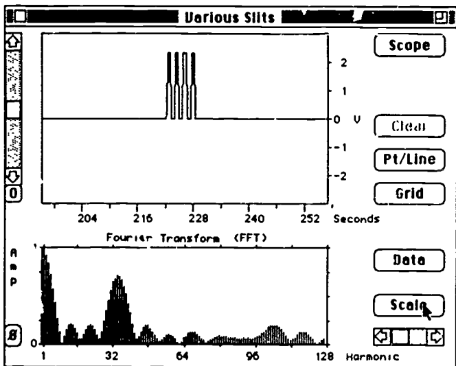
Figure 8. When a laser beam passes through a slit structure, it makes the resulting diffraction pattern in the Fourier transform of the slit pattern. Here we made a four-slit structure using a two-volt battery and a switch. The Fourier transform accurately resembles the four-slit diffraction pattern seen and recorded in our diffraction laboratory experiment.
