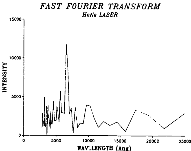
Figure 1. Fast Fourier transform of a HeNe laser.
