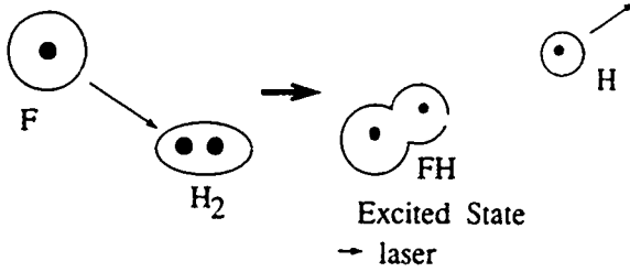
Figure 9. The reactions involved in the fluorine-based chemical laser are typical of those requiring computer performance approaching the teraflop range.
