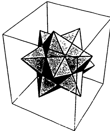
Figure 10. A 3-dimensional plot of a stellated dodecahedron.
