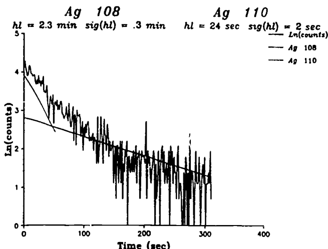
Figure 7. Decay curve for Ag^{108} and Ag^{110} .
