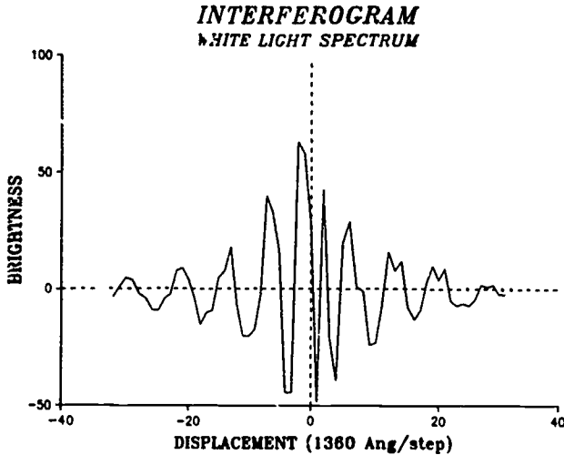
Figure 2. Interferogram of white-light spectrum.
