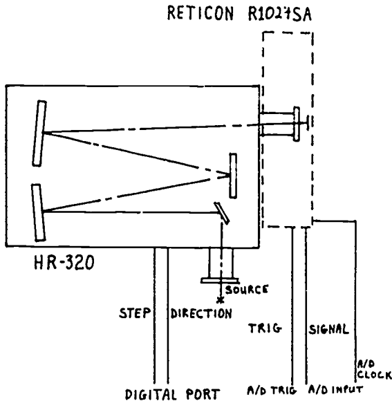
Figure 8. Spectrometer with reticon detector.
