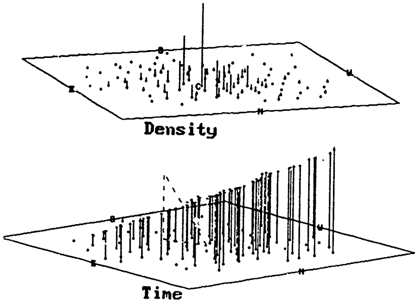
Figure 1. Cygnus experiment online displays of electron density and relative arrival time.
