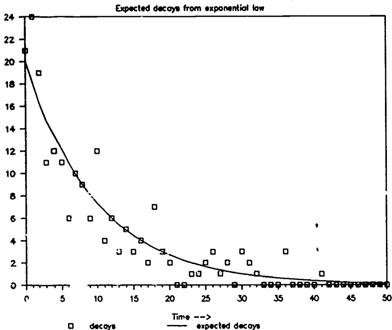
Figure 1. Histogram of the lifetimes realized in 200 runs of the radioactive decay simulation, compared to the average behavior expected in large numbers of runs
