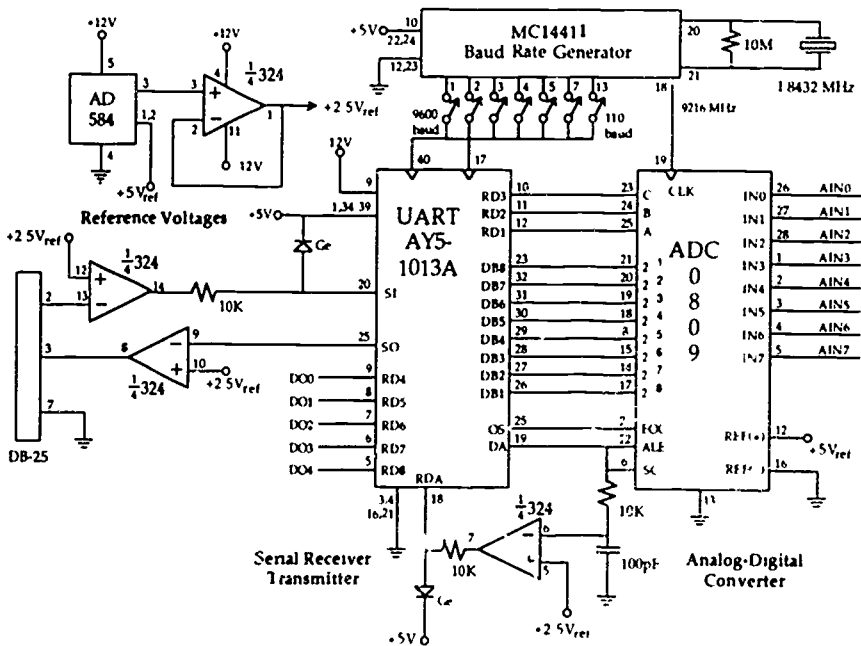
Figure 1. A schematic of the universal analog lab. The 0809 is an 8-channel, 8-bit analog-to-digital converter. When the universal serial asynchronous receiver/transmitter (USART) receives a complete byte from the computer, it starts the analog-to-digital converter, using one of the eight analog inputs. When the conversion is complete, the USART is signaled to transmit the resulting 8-bit value back to the computer.
