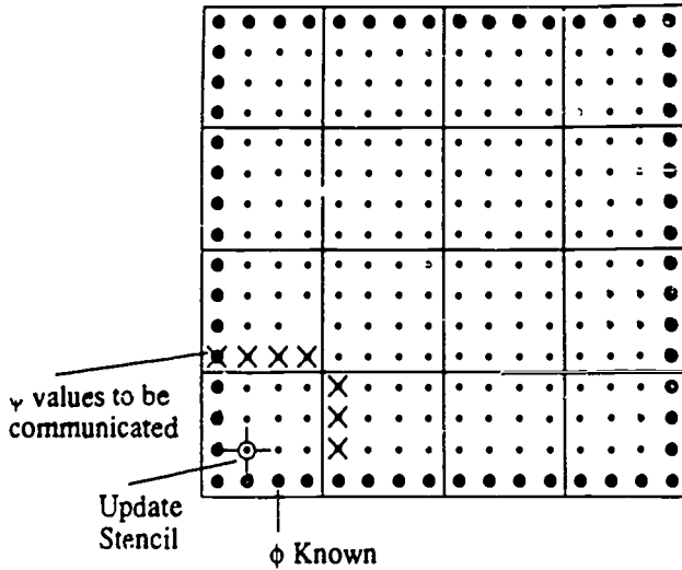
Figure 5. The role of processor 0 (in the bottom left corner). The update stencil equation 1 is applied to each point at which \phi is unknown. In order to update the grid points on the upper and righthand boundaries, processor 0 must communicate with the processors above and to the right of it.
