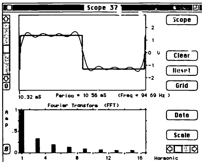
Figure 7. Analysis of an experimental square wave. We grabbed the square wave from an HP oscillator, selected one period of the wave, and then reconstructed the wave from the first four nonzero harmonics. Notice that the even harmonics are missing and the odd ones go as 1/N . When you click on the button labeled \emptyset , the phases and then the intensities of the Fourier components are displayed.
