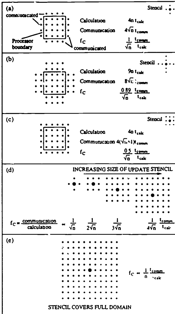
Figure 7. The effect of differing stencils on the communication overhead f_C . For the stencils in panels a, b, and c, f_C is proportional to 1/\sqrt{n} , where n is the number of grid points per processor. As the stencil size increases (see panel d), f_C decreases, until when the stencil covers the full domain of the problem (panel e), f_C is proportional to 1/n . This corresponds to a long-range force problem.
