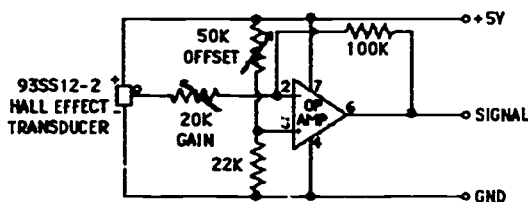
Figure 1. Variable-gain Hall Effect amplifier.
