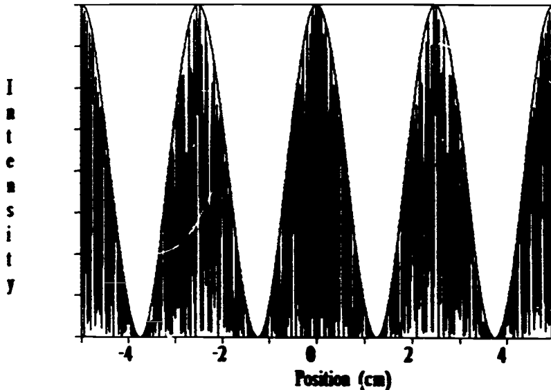
Figure 4. Intensity pattern from a Young's slits computation. The distance between the slits is 20\ \mu ; wavelength is 500\ \text{nm} ; and the distance from slit to screen is 1\ \text{m} . The pattern is shown for one time. The envelope function that reflects the time average is also plotted.
