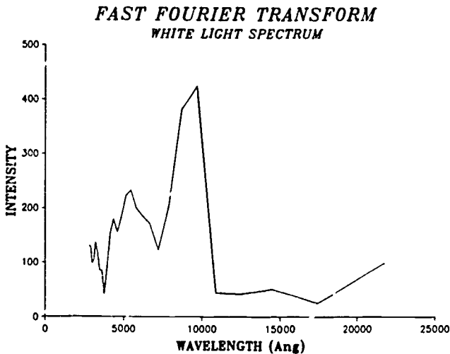
Figure 3. Fast Fourier transform of white-light spectrum.
