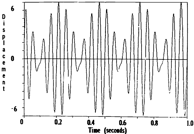
Figure 3. Superposition of two waves whose frequencies are 20 and 24 Hz. Their corresponding amplitudes are 4 and 3.
