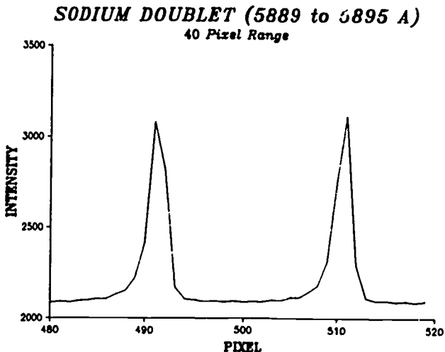
Figure 10. Visible spectrum for Na showing the doublet lines, with an expanded scale.
