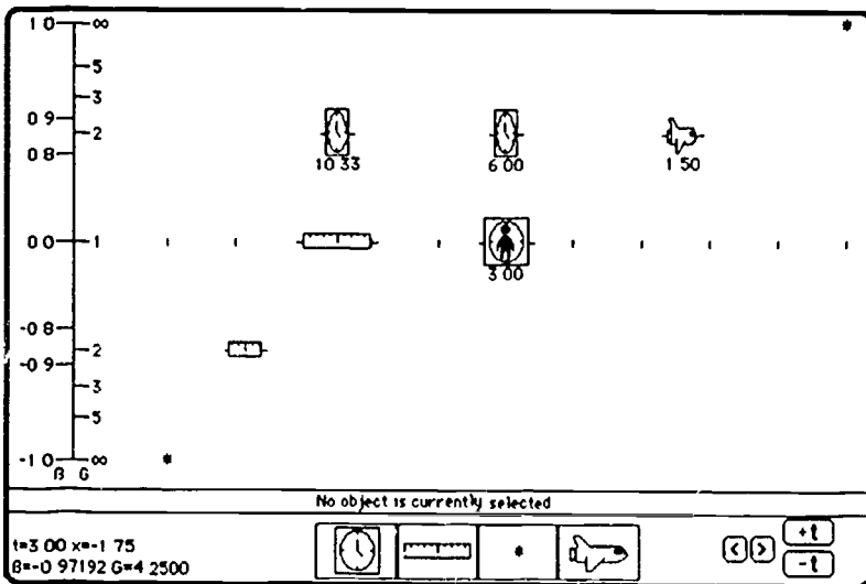
Figure 1 Highway display in the Spacetime program, showing clocks, rods, light flashes, and the shuttle (the only object that can change lanes). In this version the operator drags objects onto the highway from "object wells" at the bottom. Two scales at the left calibrate the velocity \beta = v/c of the different lanes and the corresponding time-stretch factor \gamma (printed as G ). Mouse buttons at the lower right step time forward and backward and move the screen right and left. Printed at the lower left are frame time and highway location of the cursor (not shown).
