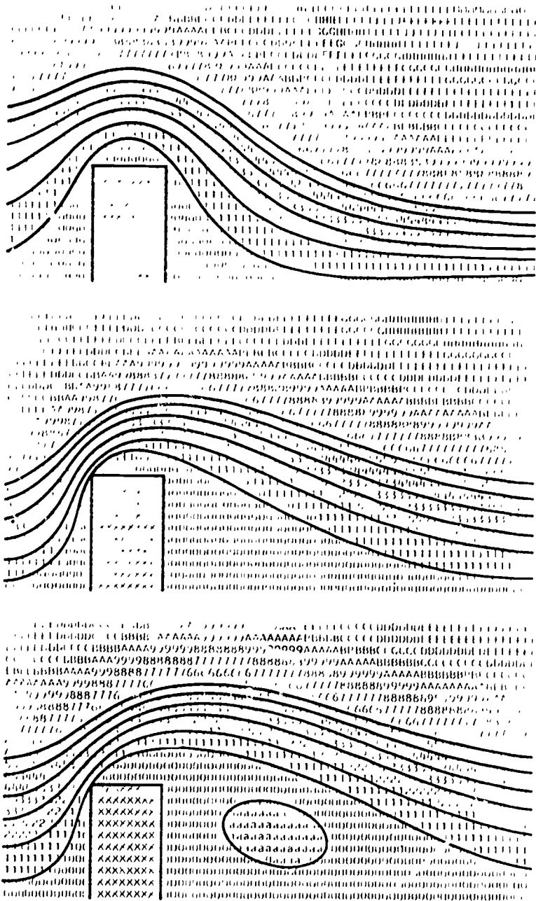
Figure 2. Streamlines for a viscous fluid flowing around a rectangular plate at various velocities. The direction of flow is from the left, and each pattern is reflection-symmetric about the lower edge. Note particularly the hydraulic “jump” above the plate, the laminar flow at low velocity (top pattern), the increasing separation of the flow from the rear of the plate at higher velocities (middle pattern), and the vortex behind the plate at the highest velocity (bottom pattern).
