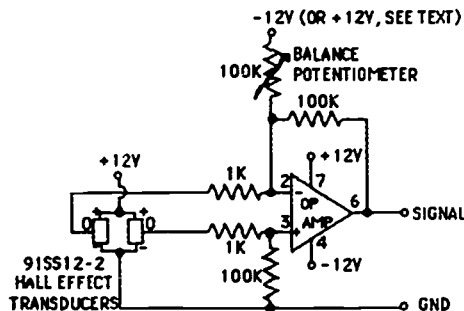
Figure 2. High-gain Hall Effect amplifier.
