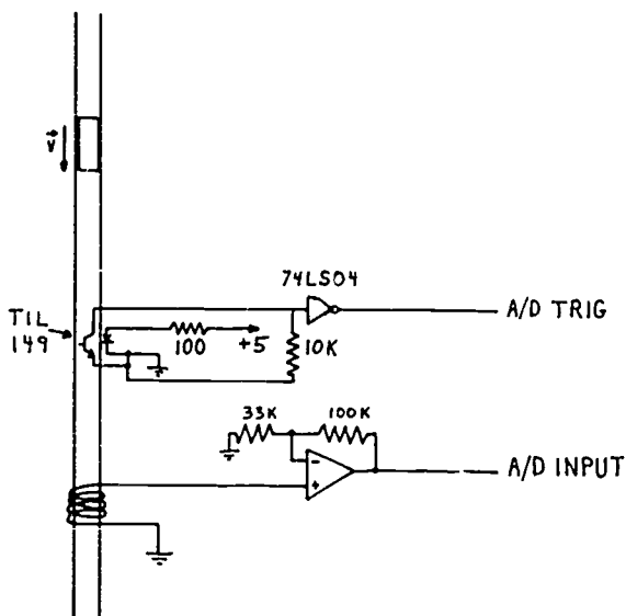
Figure 11. Apparatus and circuit diagram to measure Faraday's law.
