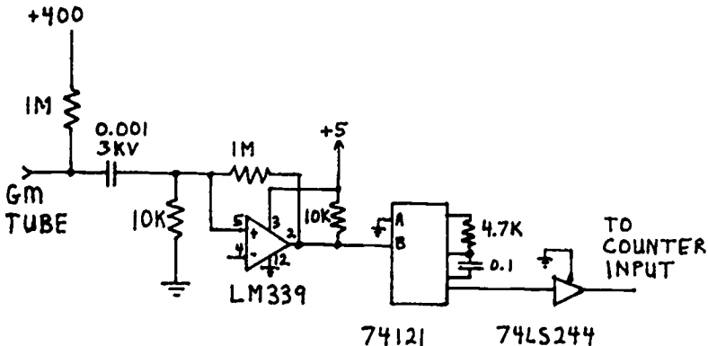
Figure 5. Circuit diagram for a Geiger-counter interface.
