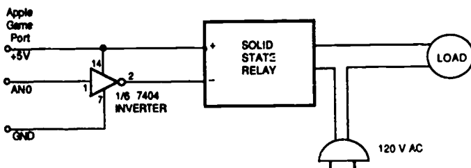
Figure 10. Apple II AC control circuit.
