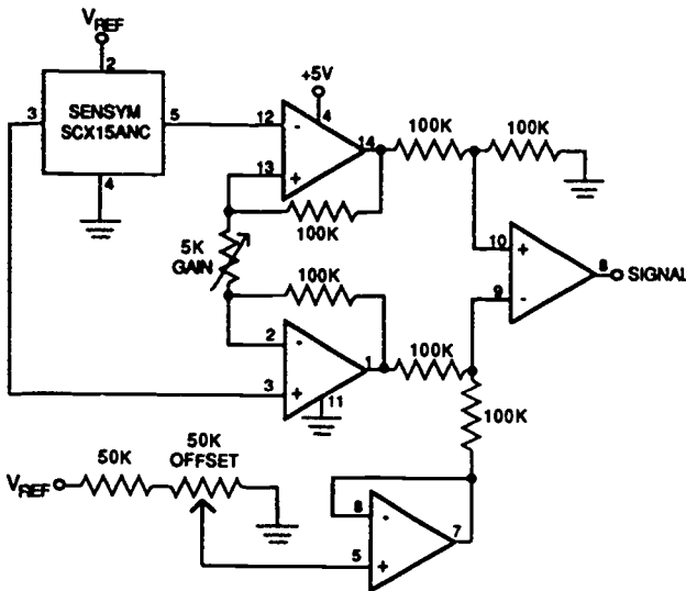
Figure 8. A variable-gain pressure sensor circuit.
