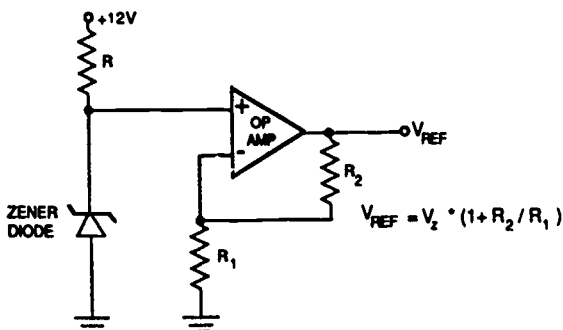
Figure 9. Voltage reference circuit.
