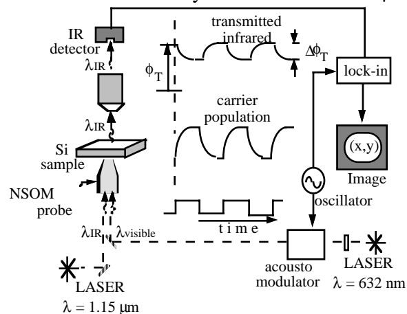
Figure 1: Schematic of the experiment that extracts information about the local dynamics of excess carriers in a semiconductor. Left side: optical path of the IR radiation through the microscope. Center: A timing diagram of the process. The visible light creates carriers which decay over their lifetime. An increase in carrier population causes a decrease in the IR transmission. Right: Diagram of the synchronous detection of the transmitted IR signal. An image is constructed as the probe is scanned across the sample.
