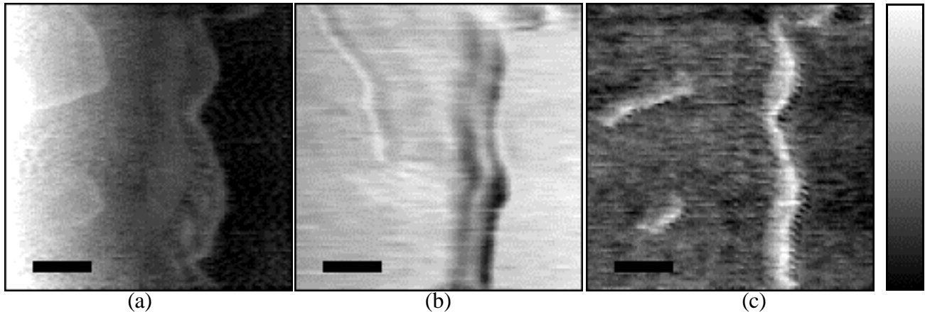
Figure 2: Three images show the same 20 micron square region of an oxygen terminated silicon surface with different contrast methods. The bars are 4 microns long. (a) A topographic image with a 240 nm vertical range -- white higher. (b) The infrared transmission (0.71 nW range with a ~80.0 nW dc background subtracted) shows regions of contrast, white more intense. (c) The time-resolved image of the change in IR amplitude as the visible light is switched reveals regions near multiple step defects which have a faster recombination rate (white). The range is 0.063 nW.
