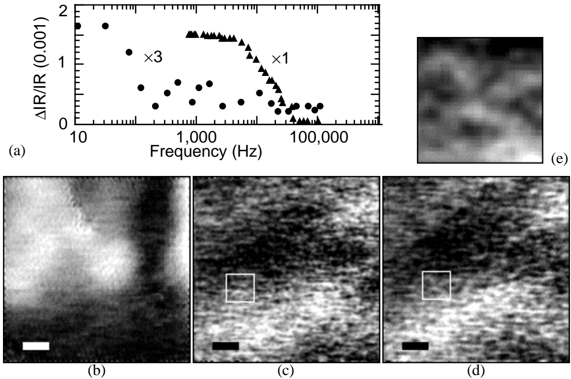
Figure 3: (a) Plots of the relative IR signal change vs. the visible light switching frequency are shown for two different samples. The samples with data as triangles and circles have effective lifetimes estimated from the knee of 20 \mu sec and 1.6 msec, and images shown in figure 2 and 3, respectively. (b)-(d) The effects of varying the visible light switching frequency in 7.5 \mu m square images of nearly the same area on the 'circle' sample, with 1 \mu m size bars. (b) An image of the IR signal change as the visible light is switched on and off at 100 Hz with 0.27 nW range. (c) As (b), but at a frequency of 2 kHz, 0.03 nW range. (d) At 20 kHz modulation, 0.03 nW range. (e) A detail from image (d) approximately one wavelength (of 1.15 \mu m IR) square, with 0.02 nW range. The boxes in (c) and (d) show the corresponding area.
